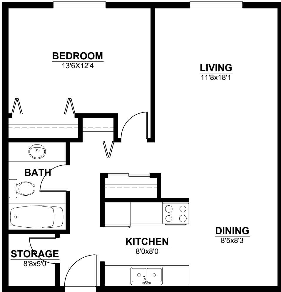
AVINLEA - 1 BEDROOM UNIT Approx. 724 SQ.FT.
